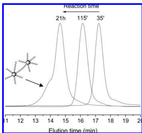
Figure 2. SEC curves as a function of reaction time for star-shaped PiBA with 12 arms (PiBA_12A_2).
