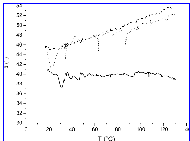
Figure 10. \delta as a function of temperature for PnBuA_blank ( \cdot \cdot \cdot ), PnBuA_M1 ( - - - ), and PnBuA_M3 ( - ).
